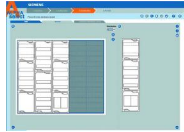
ALPHA SELECT meter cabinet equipment
