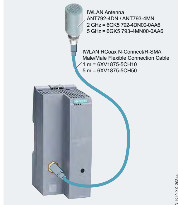
Client Module SCALANCE W722-1 RJ45
